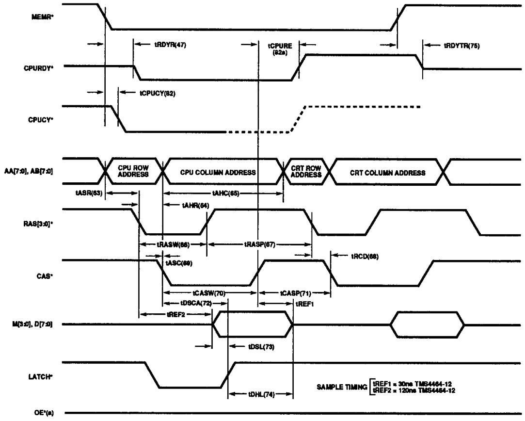
(a) Signal timing for 64K x 16 DRAM interface only.
